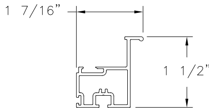
LIFT RAIL (BP4006) EXTRUDED RIGID PVC
