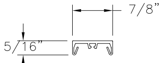
MULLION CAP (1847R) EXTRUDED RIGID PVC
