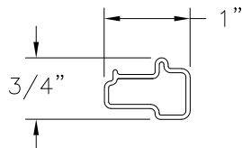
LOCK RAIL/ STILE REINFORCEMENT (204-B) ALUMINUM 6063-T5
