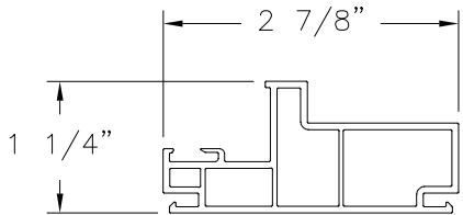
TRANSOM FRAME (BP4003) EXTRUDED RIGID PVC
