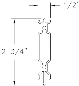
REINFORCEMENT (210-A) ALUMINUM 6063-T5
